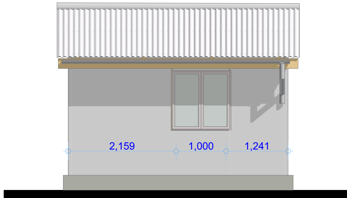
SOUTH ELEVATION
